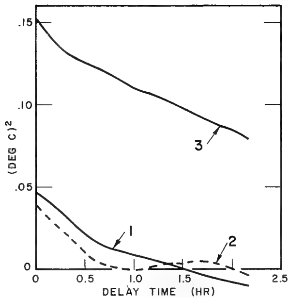
Figure 7. The temperature records of mean lagged products for three successive days, Buoy 2, at a depth of 150 ft.
